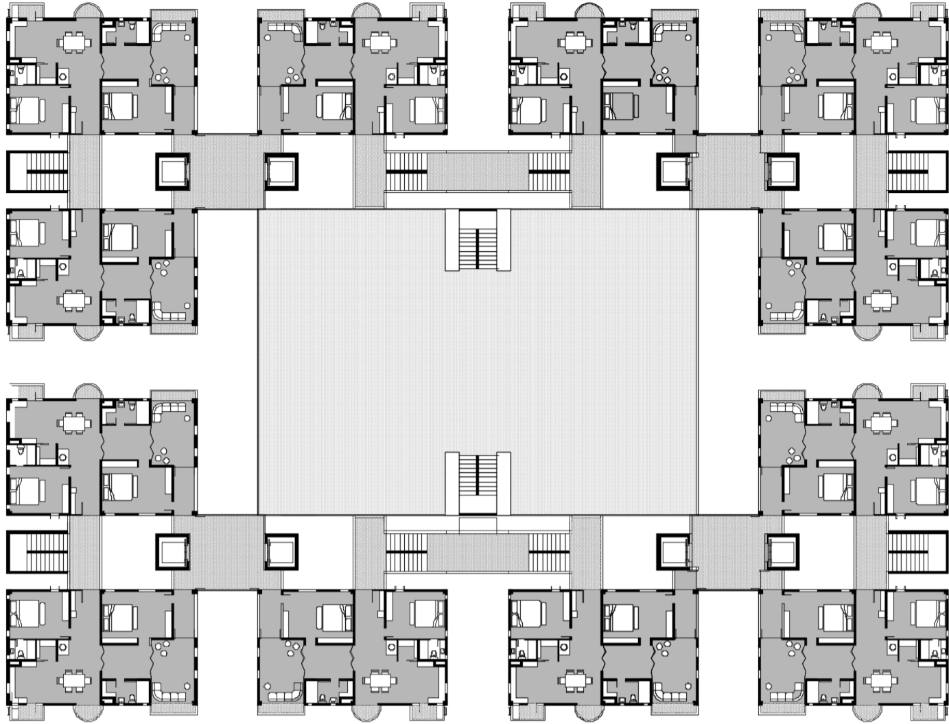
5th, 6th and 7th FLOOR PLAN
