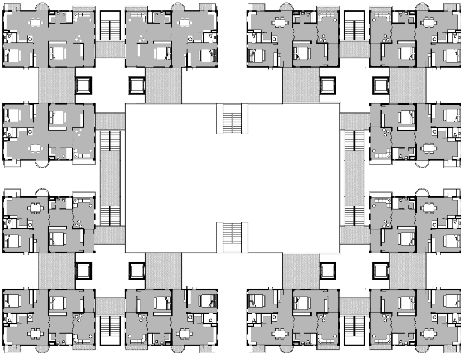
8th, 9th and 10th FLOOR PLAN
