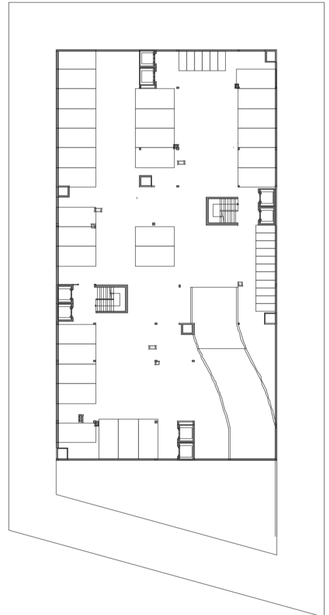
Basement Plan
