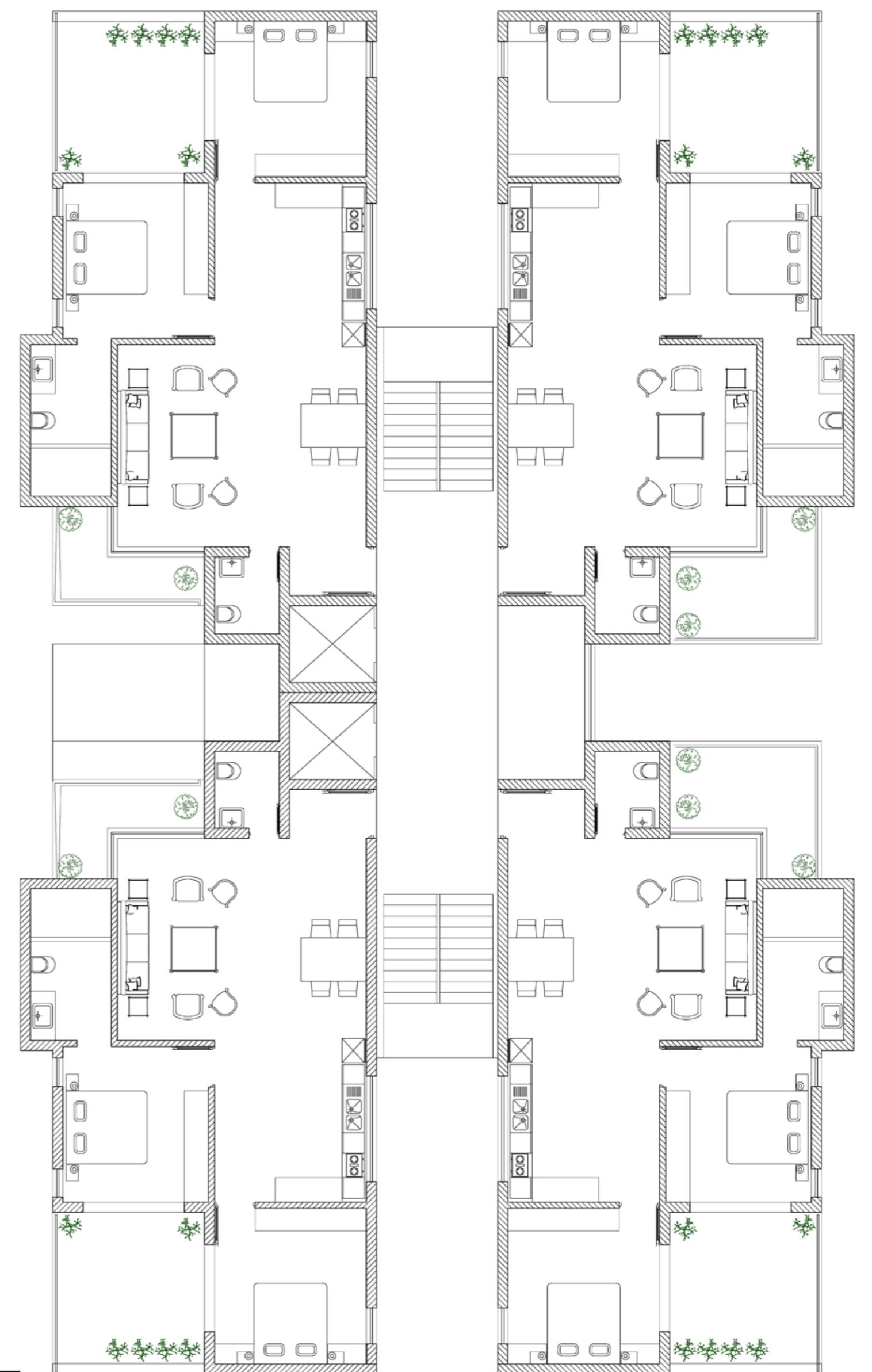
CLUSTER PLAN
