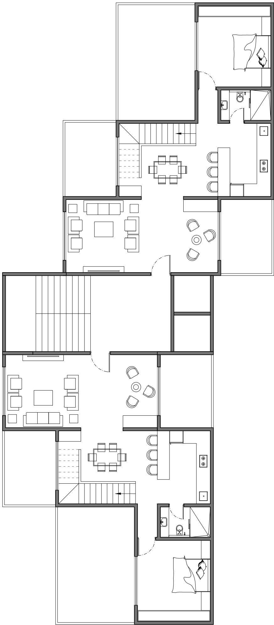
LEVEL 01
