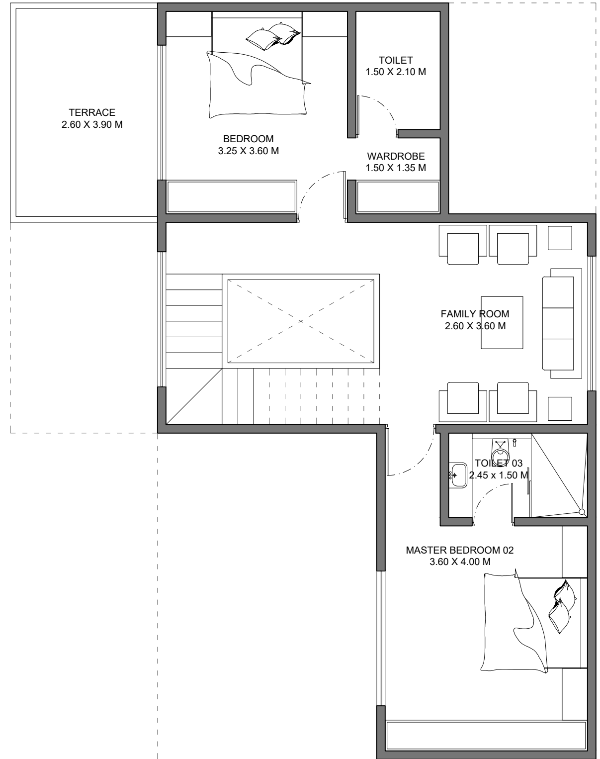
LEVEL 02
