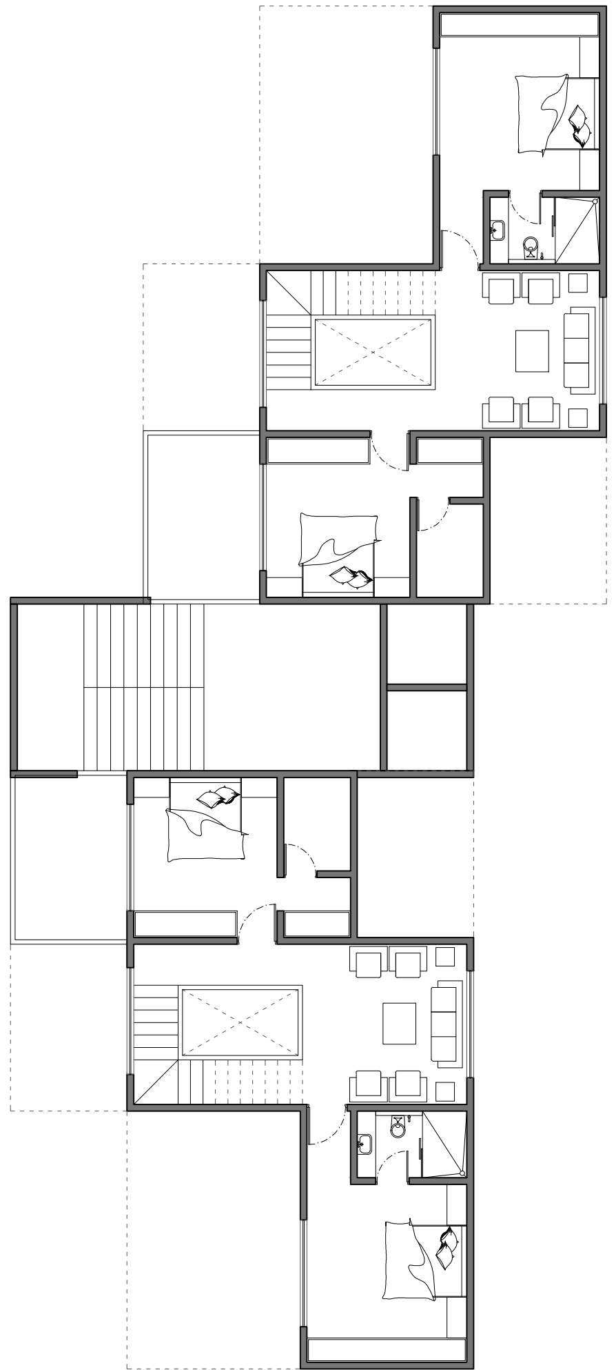
LEVEL 02
