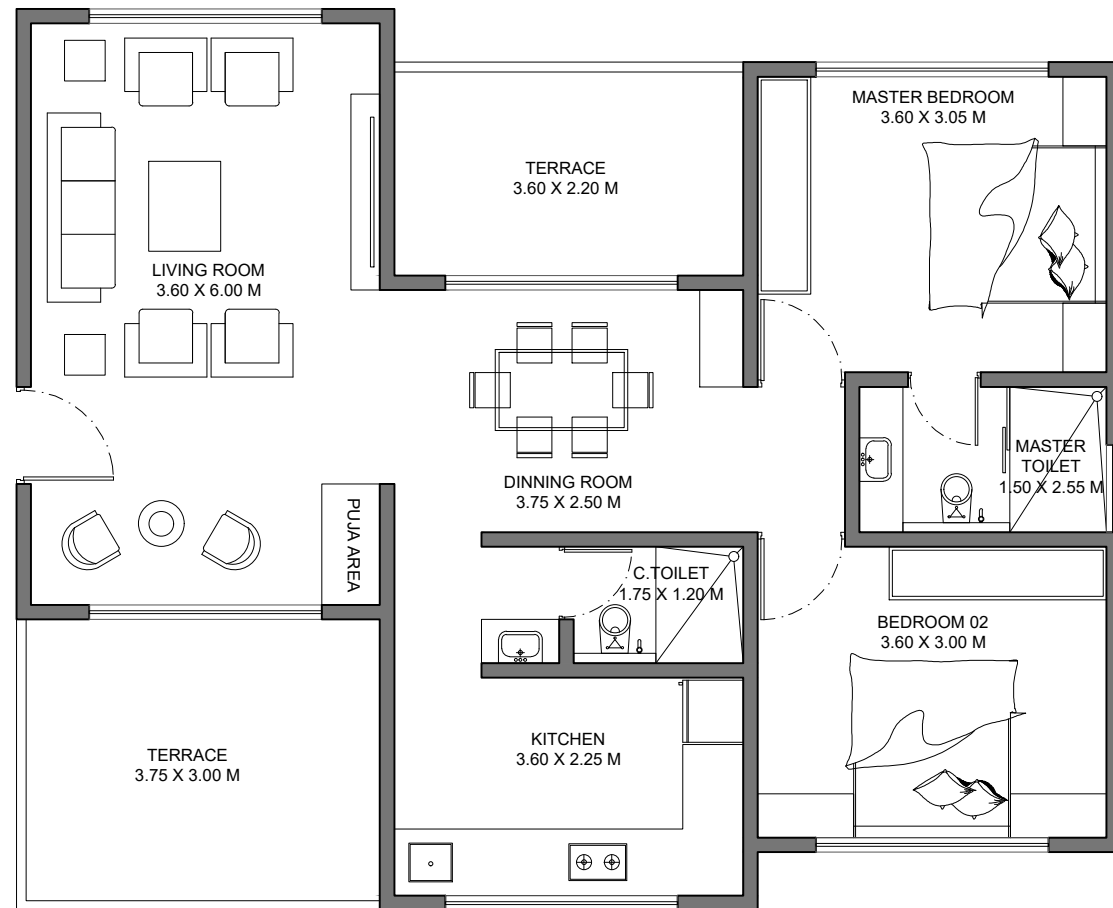
TYPICAL 2BHK UNIT PLAN : BUA - 99.08 SQ.M.
