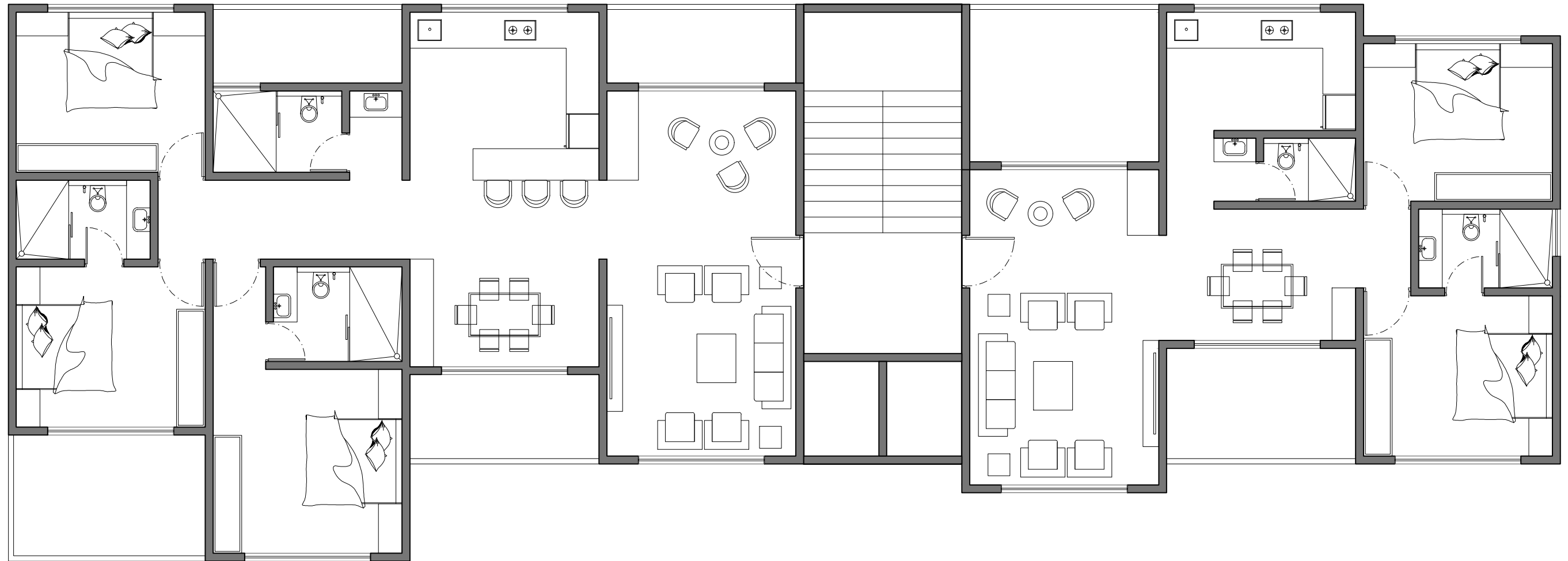
TYPICAL 2BHK & 3BHK FLOOR PLAN : BUA - 240.55 SQ.M. G+11
