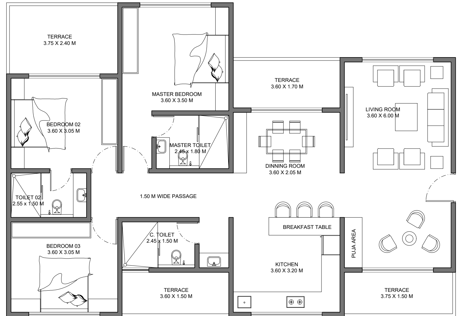
TYPICAL 3BHK UNIT PLAN : BUA - 146.71 SQ.M.
